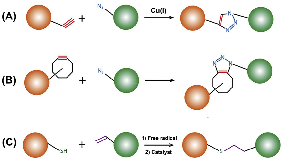
Fig. 7. Schematic illustration of reactions that best meet the criteria for a click reaction. A. Cu(I)-catalyzed azide-alkyne cycloaddition (CuAAC); B. Cu-free click cycloaddition; C. thiol-ene reaction. [183], Copyright 2011.
