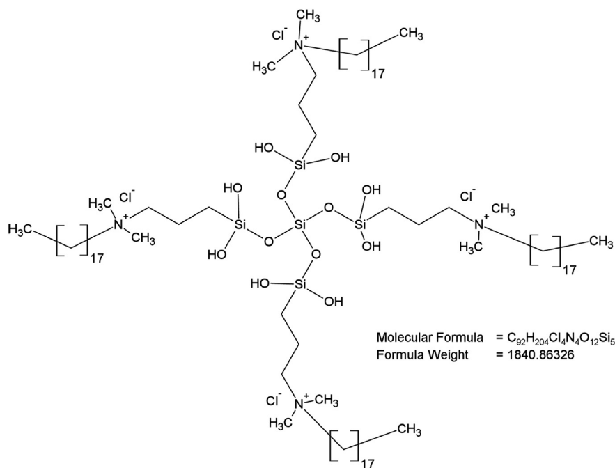
Fig. 1. Idealized chemical structure of the quaternary ammonium silane employed in the present study.
