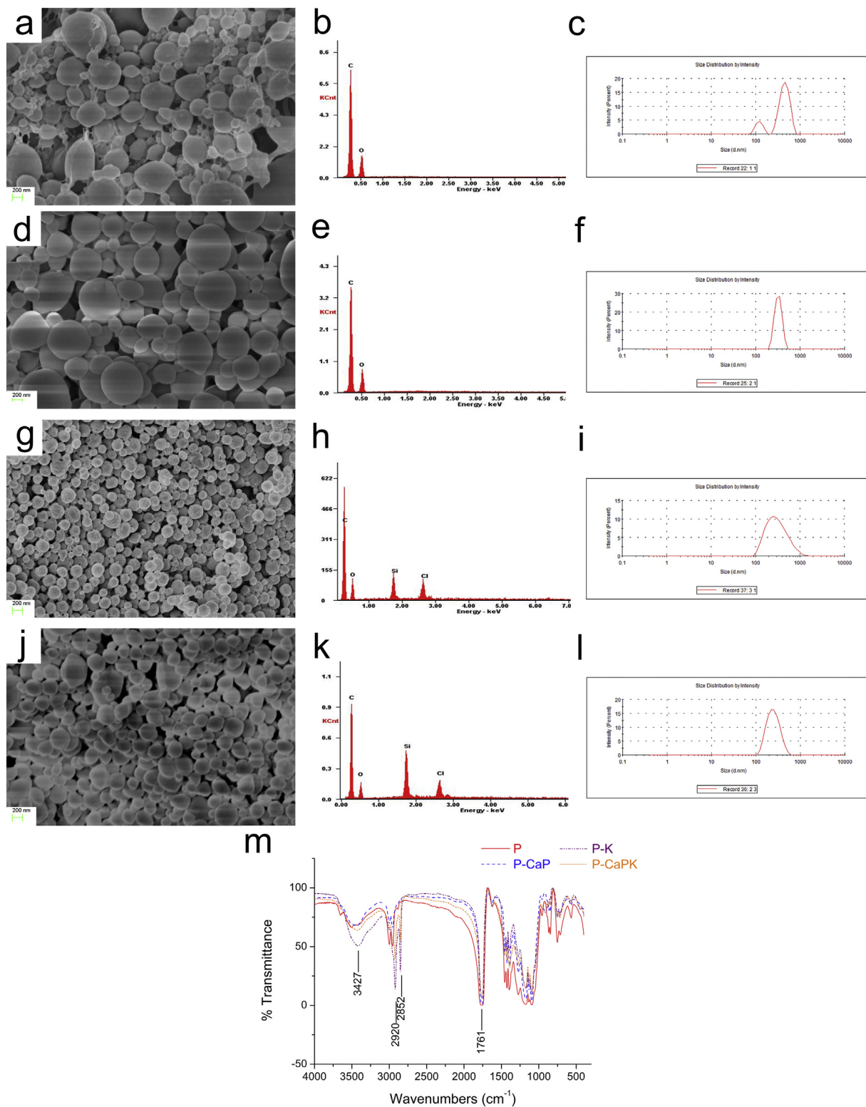
Fig. 2. Characterization of P, P-CaP, P-K and P-CaPK. a. SEM image of P; b. EDS analysis of P; c. size distribution graph of P; d. SEM image of P-CaP; e. EDS analysis of P-CaP; f. size distribution graph of P-CaP; g. SEM image of P-K; h. EDS analysis of P-K; i. size distribution graph of P-K; j. SEM image of P-CaPK; k. EDS analysis of P-CaPK; l. size distribution graph of P-CaPK; m. FTIR spectrum of P, P-CaP, P-K and P-CaPK.
